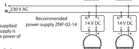
Figure 3. Each fitting is connected to a separate RGB controller. Possibility of connection to a typical 2-wire installation.
