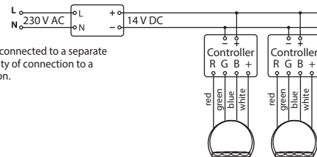
Figure 4. Fittings attached to the central RGB controller. 4-wire installation is required. Power supply adjusted to the total power of fitting and RGB controller. The power supply is chosen according to the total power of fittings and controllers.
