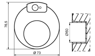
02 PIR motion sensor
