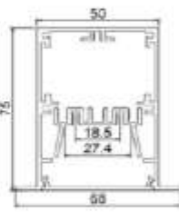
NTALBH-50R RECESSED
