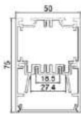
NTALBH-50-D DOWN
